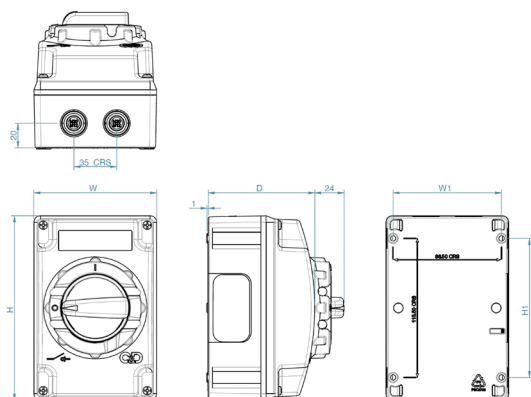
Size EA
